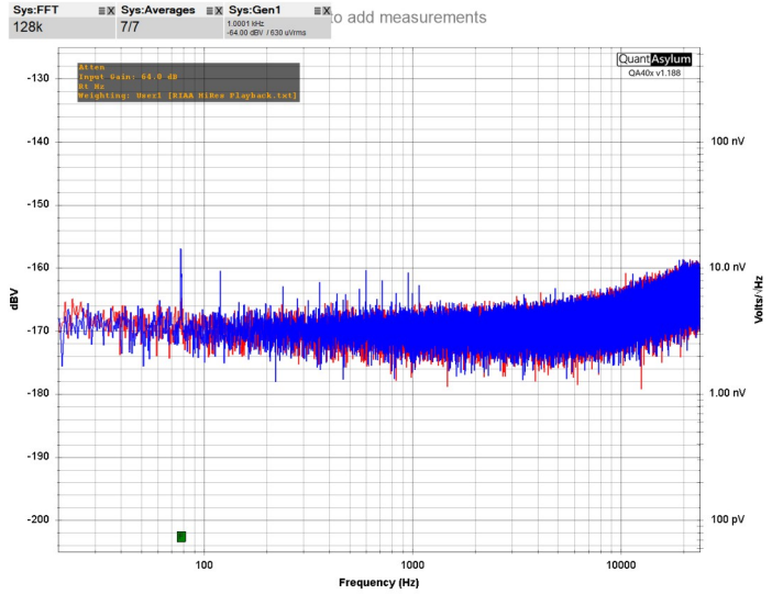
Radiance noise floor with inputs grounded
