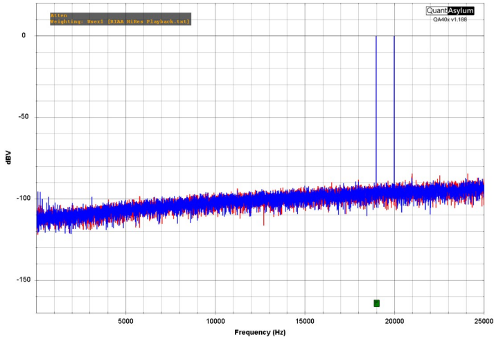
Radiance Intermodulation Distortion, 50dB gain
